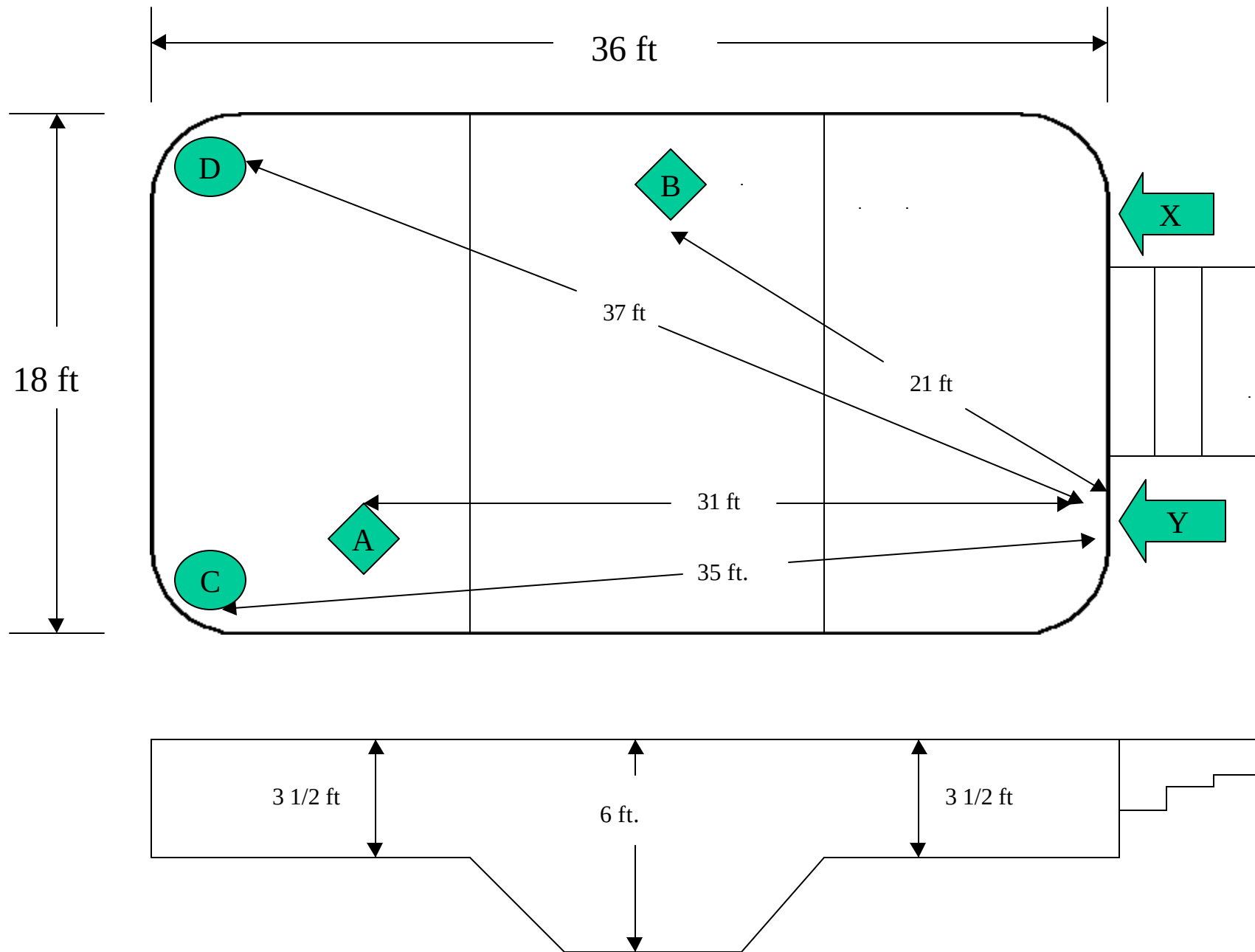
Figure B2. Sensor Locations and Water Entry Points
