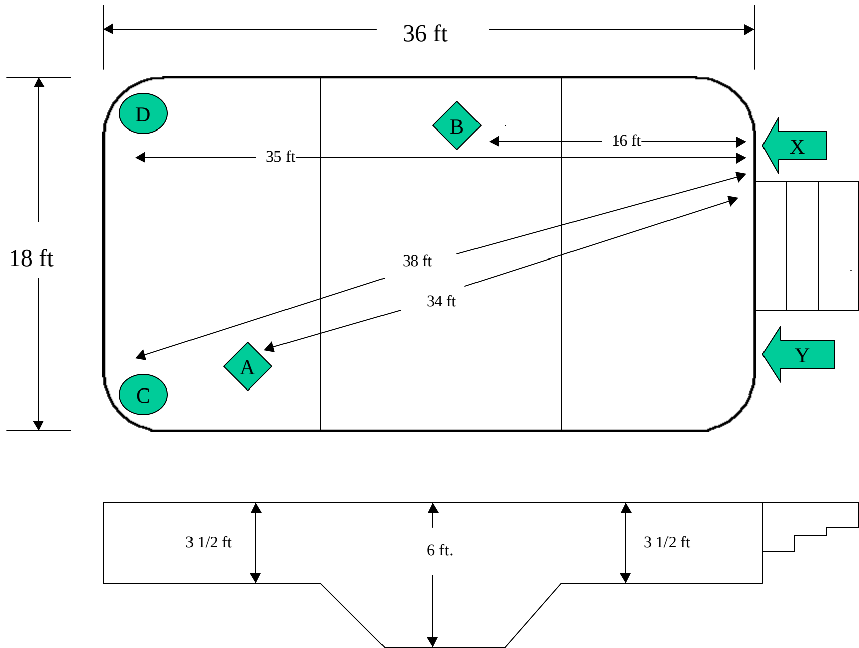
Figure B1. Sensor Locations and Water Entry Points
